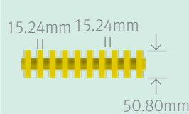
Elevation View
